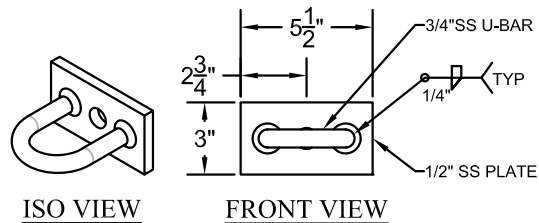
SINGLE STUD BOLT THROUGH WALL ANCHOR BTWA.0503
