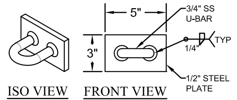
WELDABLE WALL ANCHOR WWA.0503
