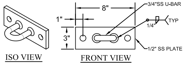
TWO STUD CIP/ADHESIVE WALL ANCHOR AWA.0803
