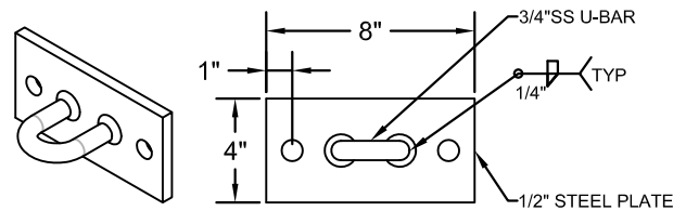
TWO STUD CIP/ADHESIVE WALL ANCHOR AWA.0804
